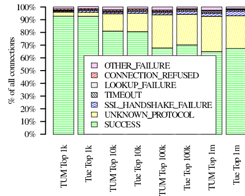
Figure 4: TLS/SSL connection errors for Tue-Nov2009 and TUM-Apr2011 scans, in relation to Alexa rank.
