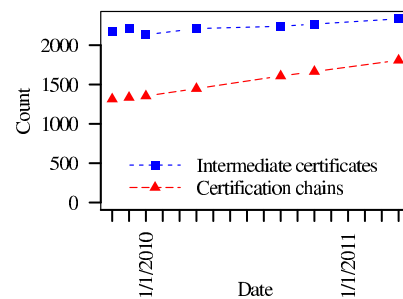
Figure 14: Temporal development of the number of distinct intermediate certificates (squares) and the number of distinct certification chains (triangles) across the scanning data sets.
