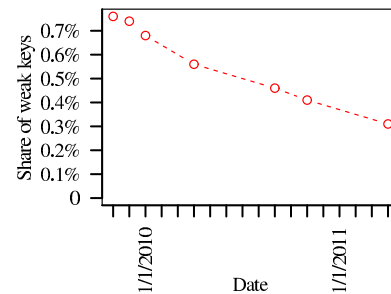
Figure 12: Debian weak keys over the course of 1.5 years in the scans of the Alexa top 1 million.
