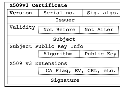
Figure 1: Schematic view of an X.509v3 certificate.
