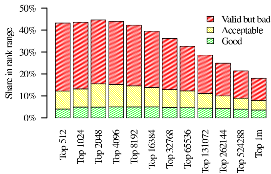
Figure 16: Certificate quality in relation to Alexa rank.
