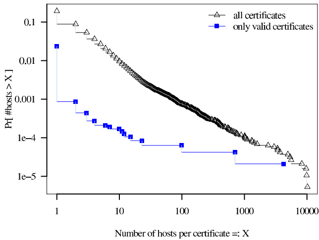
Figure 6: Certificate occurrences: CCDF for number of hosts per distinct certificate.
