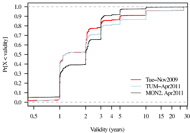
Figure 13: Comparison of certificate validity periods.
