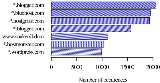
Figure 7: Domain names appearing in subjects of certificates most frequently used on many hosts.
