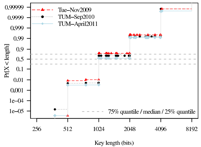
Figure 11: Cumulative distribution of RSA key lengths. (Note the unusual atanh scaling (double-ended pseudo-log) of the y axis.)
