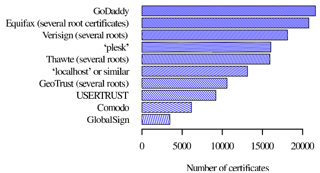
Figure 15: Top ten of issuers in TUM-Apr2011.
