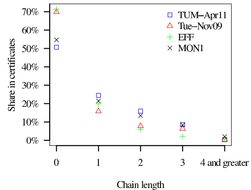
Figure 9: Chain characteristics for two scans, one monitoring run, and the EFF data. If no intermediate certificates are sent, the chain length is 0.
