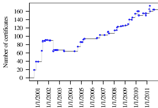
Figure 3: Growth of the NSS/Mozilla Root Store.
