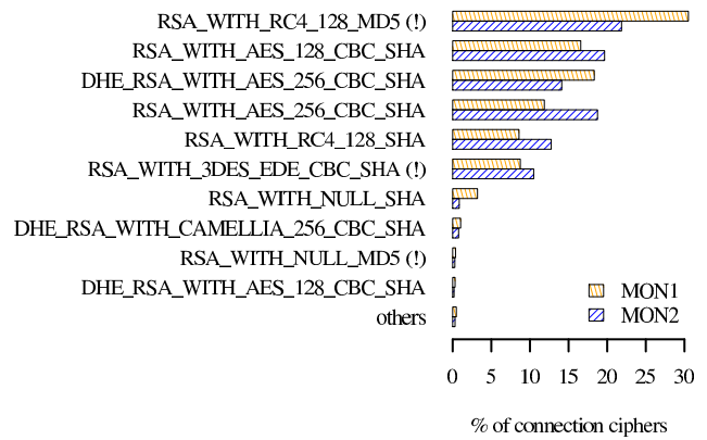
Figure 5: Top 10 chosen ciphers in passive monitoring data.
