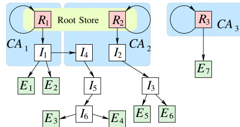
Figure 2: X.509 certificate chain examples.
