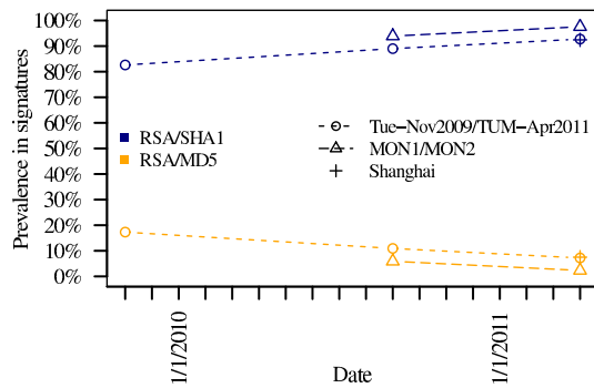
Figure 10: Popular signature algorithms in certificates.
