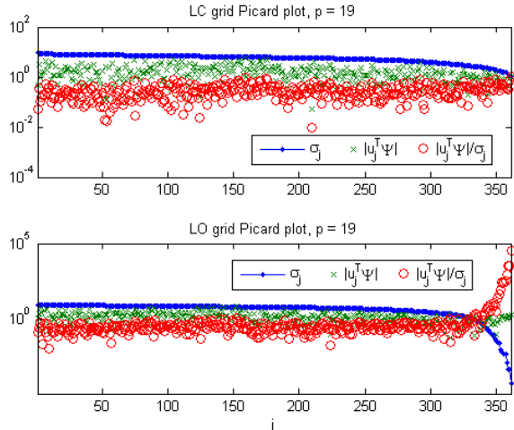
Figure 1: Sample Picard plots for closed (top) and open (bottom) grids.
