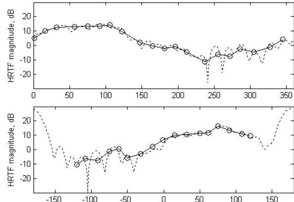
Figure 2: KU-100 manikin HRTF variation along equator (top) and along a circle in frontal plane (bottom). The value on X axis is the angle around the circle. Solid line: measured HRTF (circles denote measurement points); dashed line: evaluation of spherical harmonics representation of the HRTF obtained by the LS method.
