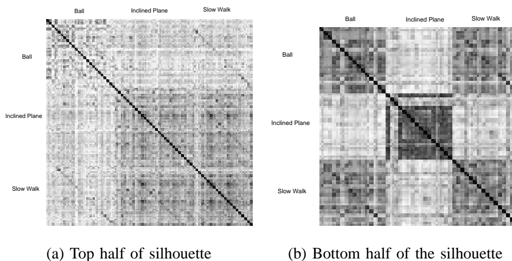
Fig. 9. Similarity matrix using the ARMA model with (a)Top half of silhouette and (b)Bottom half of silhouette
