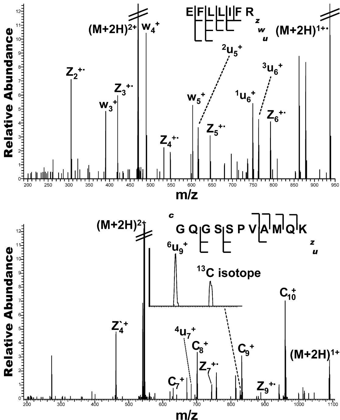
Figure 2. Top panel: Single-scan ECD mass spectrum of 2+ ions of the peptide EFLLIIR. w and u ions were manually assigned. Lower panel: Example of distant Met side chain losses in ECD of a Met-containing peptide. See text for explanation of the u ion nomenclature.
