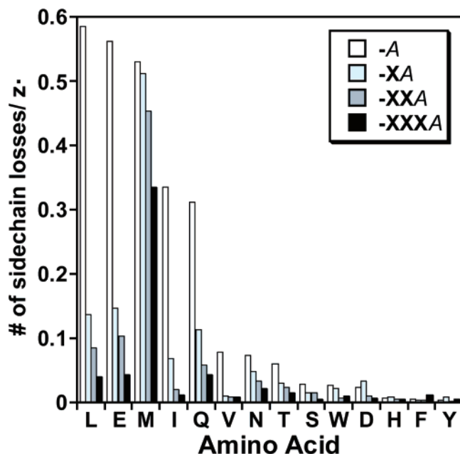
Figure 1. Frequencies of w_n ion detection relative to the presence of z_r ions determined for amino acids in different positions to the cleavage site. A is the amino acid from which the partial side chain loss occurs; X is any other amino acid except A.
