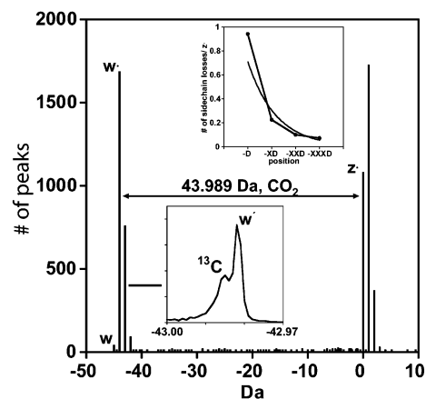
Figure 7. Same as Figure 5, but for Asp. Note that the main loss is not of \cdot\text{COOH} ( w ) but of \text{CO}_2 ( w^* ). Since the latter species is a radical, hydrogen rearrangement from the complementary fragment is possible, leading to w' (zoom-in). Inset shows exponential decay of the w'/z' ratio.
