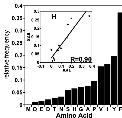
Figure 4. Relative influence of amino acids in the intermediate position X on the side chain losses from Leu_{n-2} in z_n^+ ions, where the n th amino acid is not Leu. Inset: Correlation between Leu_{n-2} and Glu_{n-2} data. The outlying amino acid is His; excluding it gives a correlation of 0.90.
