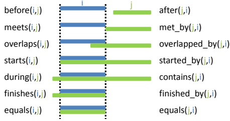
Figure 2. The base interval relations in Allen’s Interval Logic.
