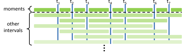
Figure 4. The space of all intervals once time is discretized. Property predicates are grounded over all moments. Event predicates are grounded over general intervals (which include moments), but only over those that are hypothesized. In our approach, time is discretized by the start and end times of hypothesized events and the times at which properties could change, given the hypotheses.
