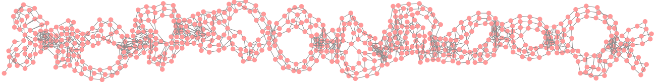
Figure 6. Ground MLN graph for 2910 frames, with 667 nodes, 2351 factors, and treewidth of 12. Nodes are ground predicates, and edges link nodes of ground predicates that appear in same formula.
