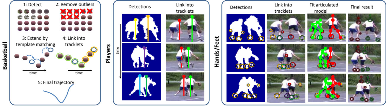
Figure 5. Tracking overview. Basketball, head, hand, and foot candidates are first detected and are then linked into tracklets.
