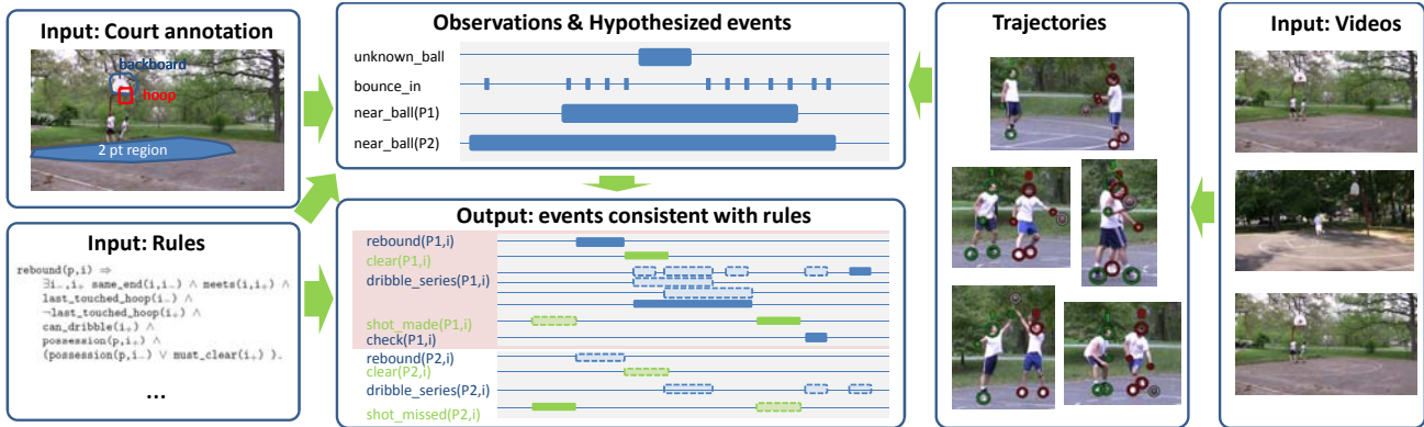
Figure 1. Framework overview. Our system obtains a set of trajectories from the input videos, which are then processed generate observations (e.g., when the ball bounced, was near a player, or was near the hoop). Based on these observations and event definitions, hypothesized event intervals are generated in a bottom-up fashion. Finally, MLN inference determines the set of hypothesized intervals that are most consistent with the observations and the formulas in the knowledge base. In this example, intervals with solid boundaries are the final detected events, while those with dashed boundaries are hypothesized intervals that were discarded by MLN inference.
