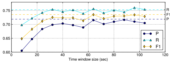
Figure 7. Performance of MLN inference with sliding windows. Dashed lines indicate full inference results from table 5.
