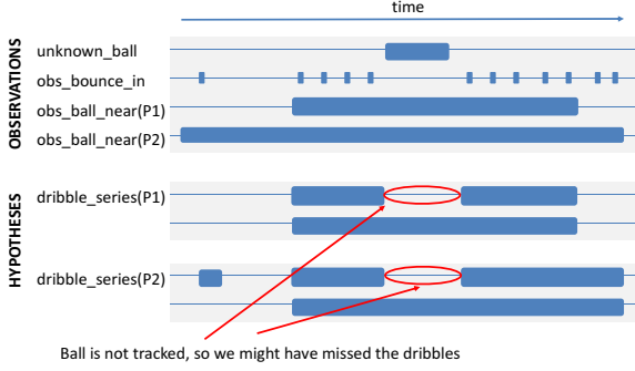
Figure 3. The bottom-up event generation module generates hypothesized event intervals from low-level observations, with the goal of achieving a high recall rate with a reasonably small set of intervals. Here, seven intervals are generated from observations for which \text{dribble\_series}(p, i) is open world (could be true).
