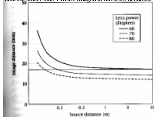
2.16. DEPTH OF FIELD OF THE HUMAN EYE. Image distance is shown as a function of source distance. The solid horizontal line shows the distance of the retina from the lens center. A lens power of 60 diopters brings distant objects into focus, but not nearby objects; to bring nearby objects into focus the power of the lens must increase. The depth of field (the distance over which objects will continue to be in reasonable focus) can be estimated from the slope of the curve.
