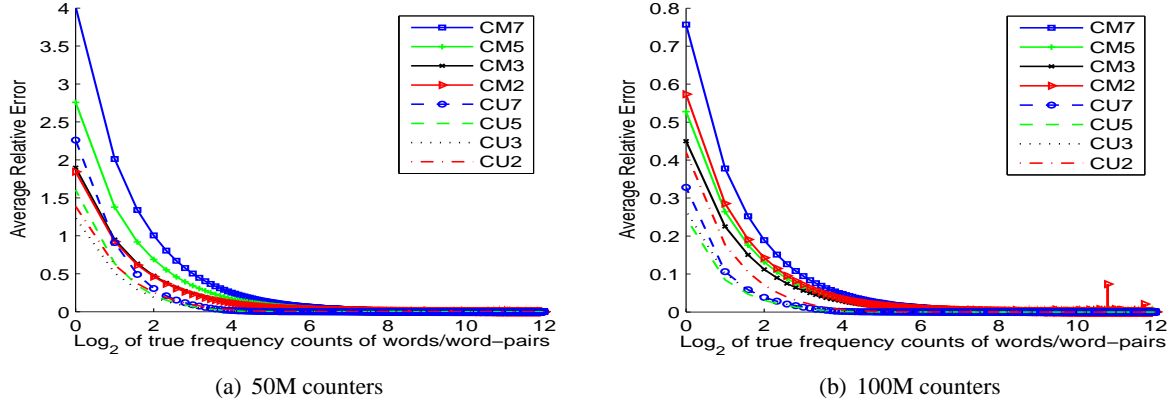
Figure 3: Comparing 50 and 100 million counter models with different (width, depth) settings. The notation CM x represents the Count-Min Sketch with a depth of ' x ' and CU x represents the CM sketch along with conservative update and depth ' x '.
