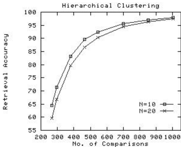
Figure 2: Retrieval accuracy with hierarchical clustering
