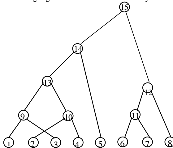
Figure 1: Cluster merging process in hierarchical clustering.
