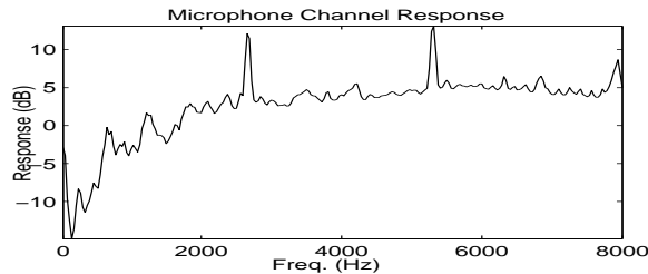
Fig. 2. Channel response applied to test data to incorporate convolutive mismatch in environments (log magnitude (in dB) vs frequency (in Hz))
