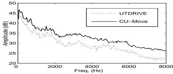
Fig. 1. Long term average noise spectra from UTDrive and CU-Move, obtained using 40 sec. duration of data (log magnitude (in dB) vs frequency (in Hz))
