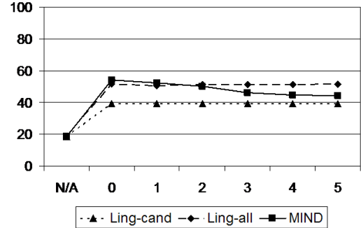
Figure 2: Percentage of Correctly Segmented Words by Different Systems for Different Threshold Values
