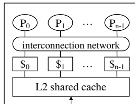
(b) shared cache only (XMT)
