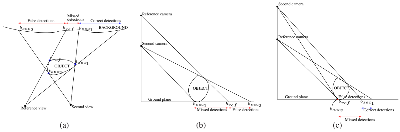
Figure 1: Problem with the algorithm from [11]. (a) Missed and false detections shown from the top view. (b) Analysis for the special case of cameras vertically aligned w.r.t. the ground plane (side view). Here the top camera is taken as reference, which causes missed detection of the whole object and false detections as shown. (c) Switching the reference camera to the lower one eliminates most of the false detections, but missed detections remain according to Eqn. 2.
