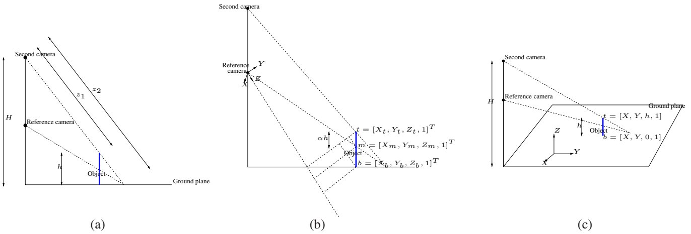
Figure 3: (a) The proportion of missed detections for a homogeneous object with negligible front-to-back depth is independent of object position. (b) Image projection in camera-centered 3D coordinate system. (c) Image projection with 3D coordinate system on the ground plane.
