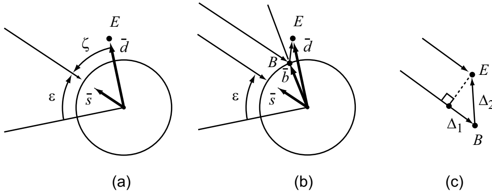
Fig. 13: Normal view of the plane defined by the vector \vec{d} from the center of the torso to the ear and the vector \vec{s} pointing to the source. (a) The “elevation” angle \epsilon . (b) The goal is to find the vector \vec{b} to the point of reflection. (c) The reflected ray travels an additional distance that is the sum of \Delta_1 and \Delta_2 .
