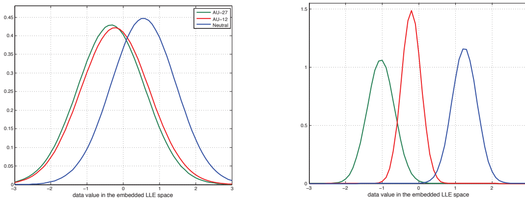
Fig. 5. Dimensionality reduction using LLE from data in the Euclidean space (left) and on the Grassmann manifold (right). Plots show the distributions of the 1D projected data separated by the classes. Better separation is seen among classes on the right.
