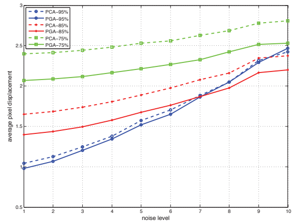
Fig. 4. PCA versus PGA bases for facial landmarks representation and reconstruction.
