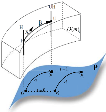
Fig. 2. Process of computing a geodesic on the Grassmann manifold by lifting it to the particular geodesic in O(m) , [20].
