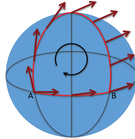
Fig. 3. Parallel transport of a vector around a closed loop on the manifold. The direction and orientation of the vector changes to match the local structure of the destination point.
