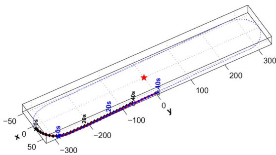
Fig. 11. Two targets follow an oval track (dotted line). The hybrid node is situated at the origin.
