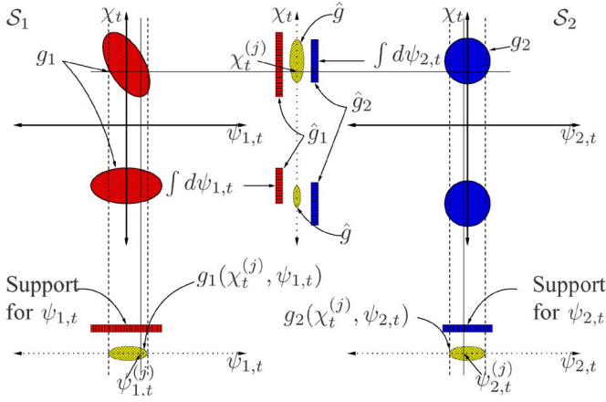
Fig. 6. The supports, g_i 's, for the posterior distribution in each state space, \mathcal{S}_i , are shown on the axes \chi_t versus \psi_{i,t} . Particles for the joint state are generated by first generating \chi_t 's from the combined supports of the marginal distributions of \chi_t . Then, the \psi_{i,t} 's are sampled from the g_i 's as constrained by the given \chi_t realization.
