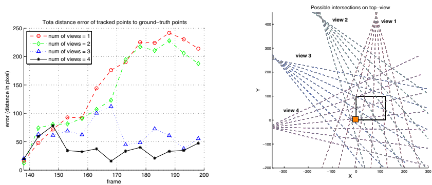
(a) Total distance error of persons' tracked (b) Homographic images all different ver-ground points to the ground truth points tical axes
