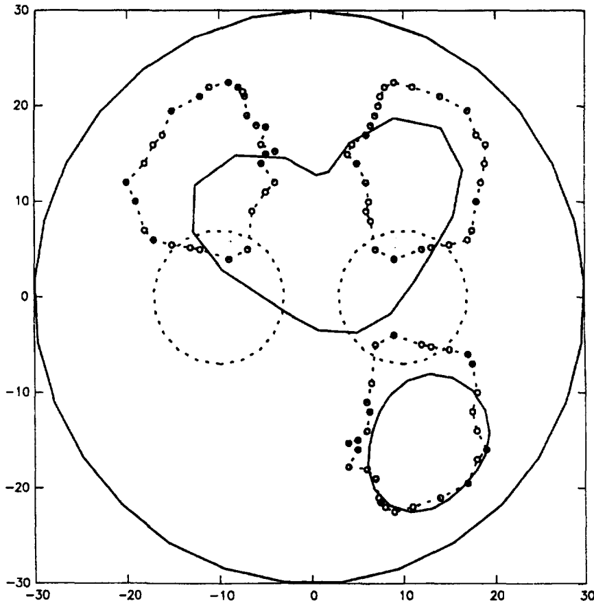
Fig. 8. EIT reconstruction of three arbitrary shapes (-○-○-) with the number of guessed shapes assumed to be two. The second computed shape spans the region occupied by two of the actual shapes (--- initial guess, — converged solution).
