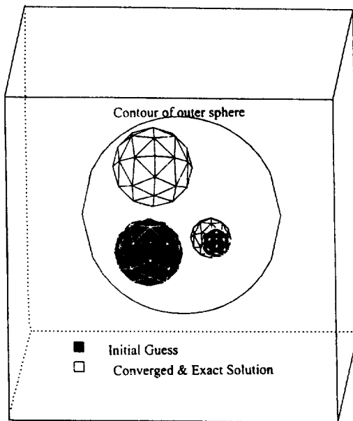
Fig. 11. Two spherical regions of zero conductivity embedded in an outer spherical region are imaged. The top figure shows a cross-sectional view with the initial guess (marked with stars), successive iterates, and the exact solution (marked with circles). A three-dimensional view of initial guess and converged solution is shown below.
