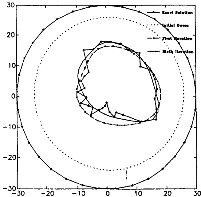
Fig. 4. EIT reconstruction of a region of zero conductivity with a jagged boundary. The inverse problem solution used a 13 parameter Legendre parametrization. Satisfactory convergence is seen, even after one iteration.
