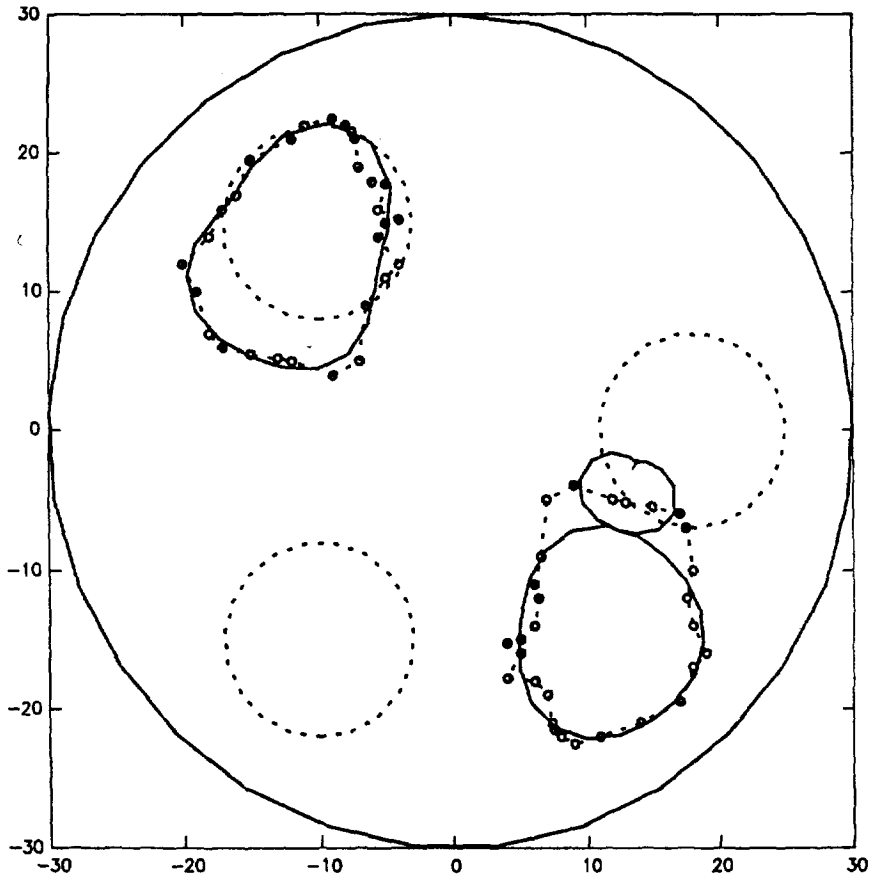
Fig. 9. EIT reconstruction of two arbitrary shapes (-o-o-) with the number of guessed shapes assumed to be three. Again, the region occupied by the actual shapes is identified by the computed shapes (--- initial guess, — converged solution).
